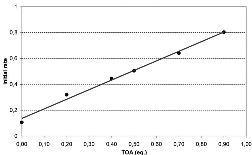
Figure 2. Rate of exchange of \alpha -H in compound 1 as a function of base concentration.
