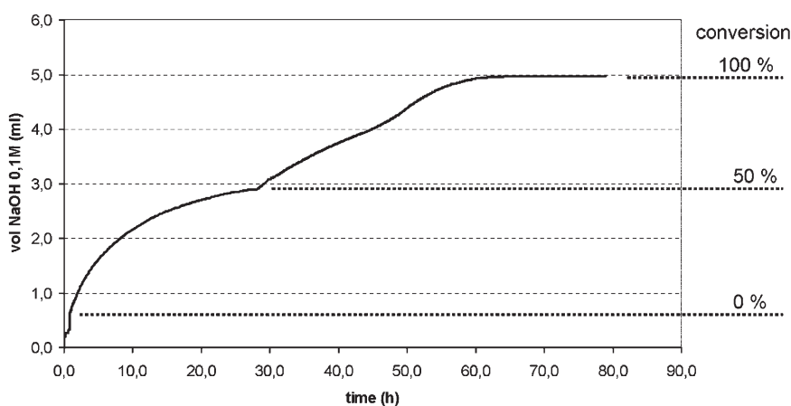
Figure 1. Time course of the DKR of compound 1 before and after triethylamine addition.
